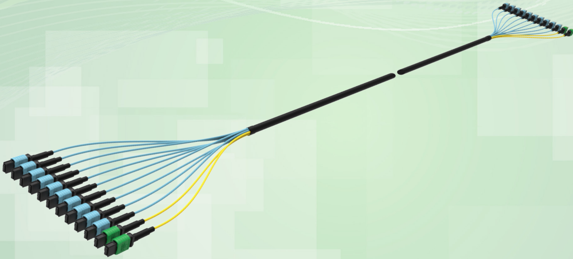
Low Loss MTP® non-pinned Trunk, 144F Hybrid, 120F OM3 & 24F OS2
